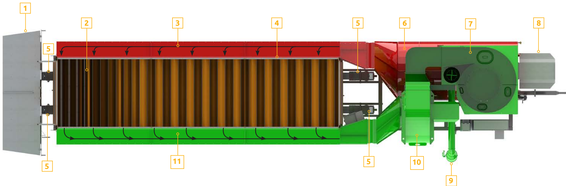
1 = 进料斗 | 2 = 缓苏仓 | 3 = 热风仓 | 4 = 干燥和冷却双坡顶风管 | 5 = 提升机 | 6 = 热风机 | 7 = 除尘器 | 8 = 燃烧器 | 9 = 降尘管 | 10 = 风机 | 11 = 排风仓
